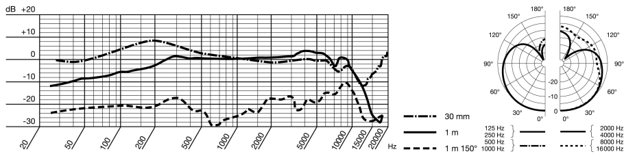
Frequency Response and Polar Diagram HSD 171, HSD 271
