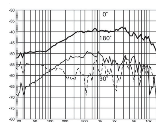
Frequency Response
