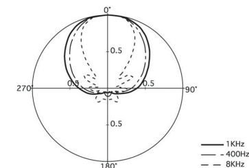
Super-Cardioid Polar Pattern
