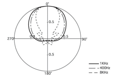
Super-Cardioid Polar Pattern
