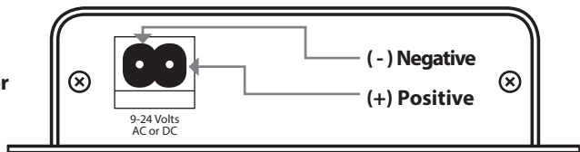
Figure 1: 5012 Power Connector DC Input Polarity
