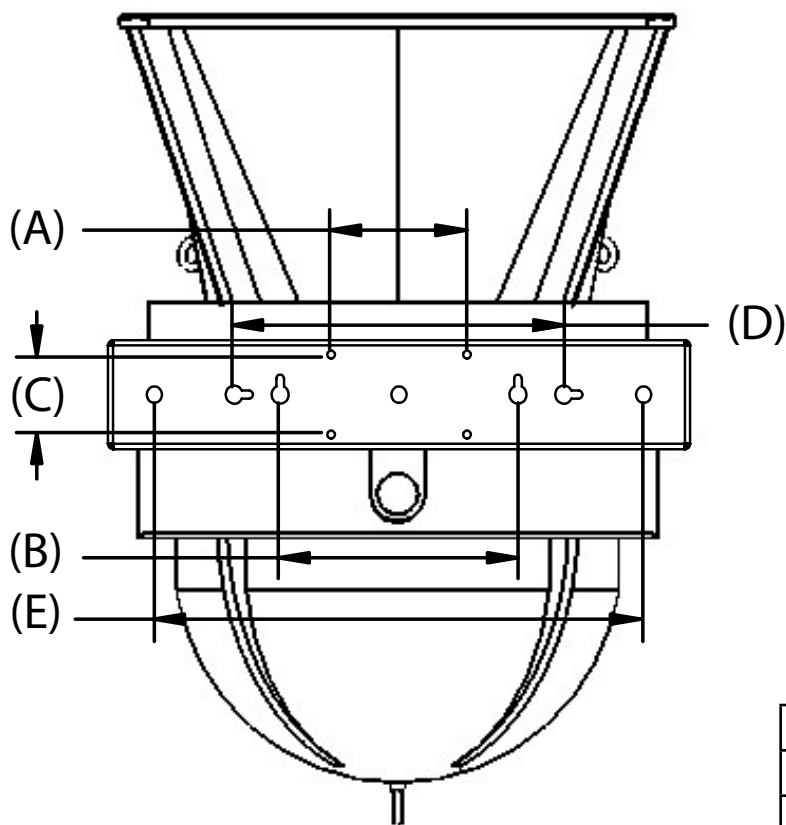
BOTTOM VIEW
