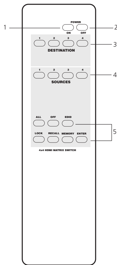
Figure 4-1. IR remote.
