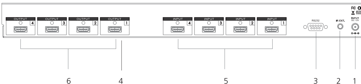
Figure 2-3. Rear panel.
