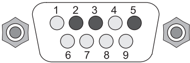
Figure 5-1. RS-232 DB9 connector.
