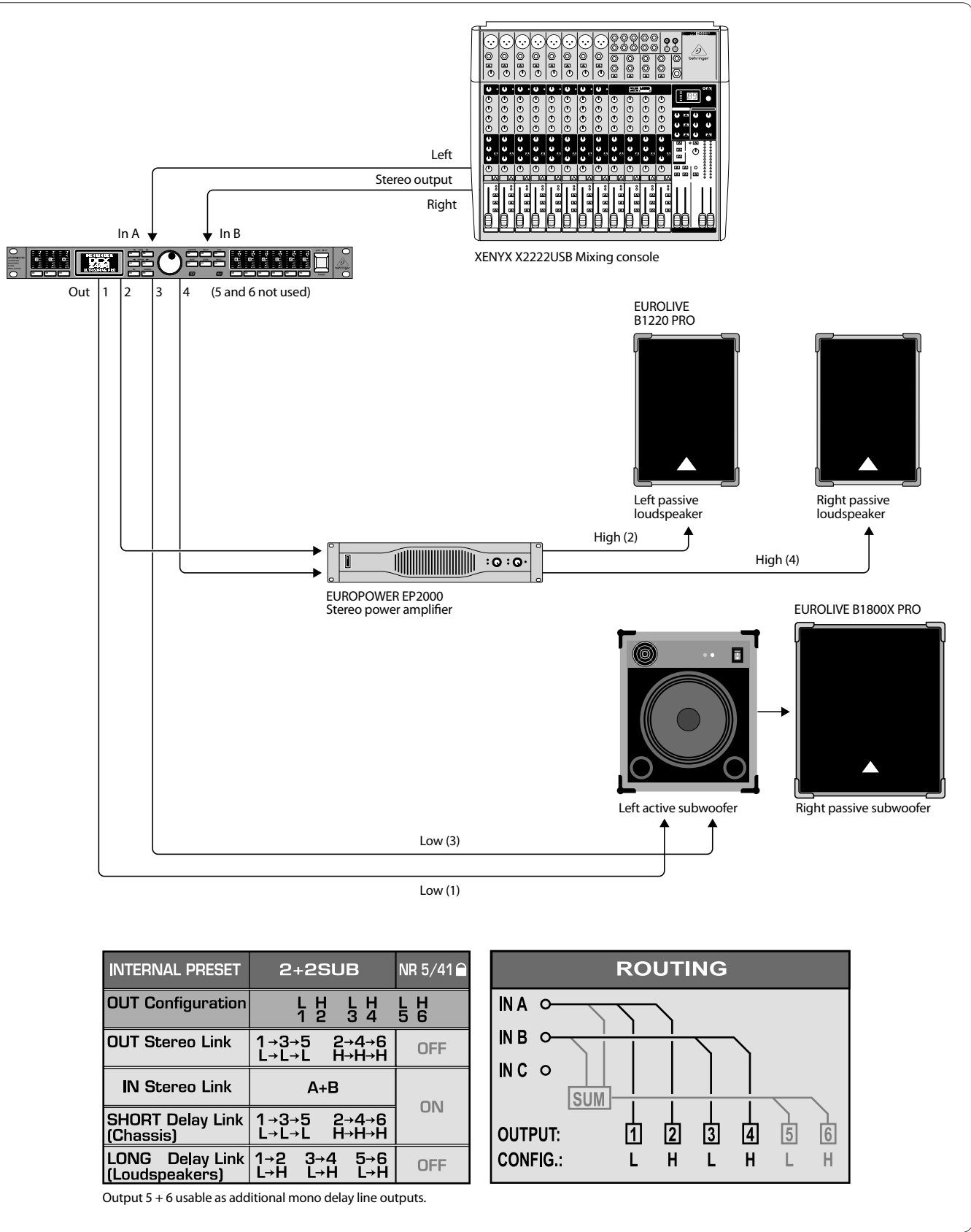
Fig. 6.5: Stereo operation plus 2 woofer cabinets
