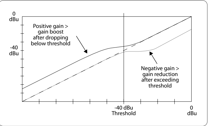
Fig. 4.36: Filter curves with gain above/below threshold
