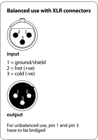
Fig. 5.1: XLR connections
