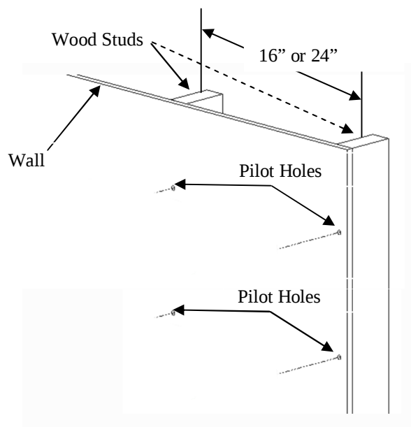
Figure 3. Wood Studs 16" or 24" Apart on Center
