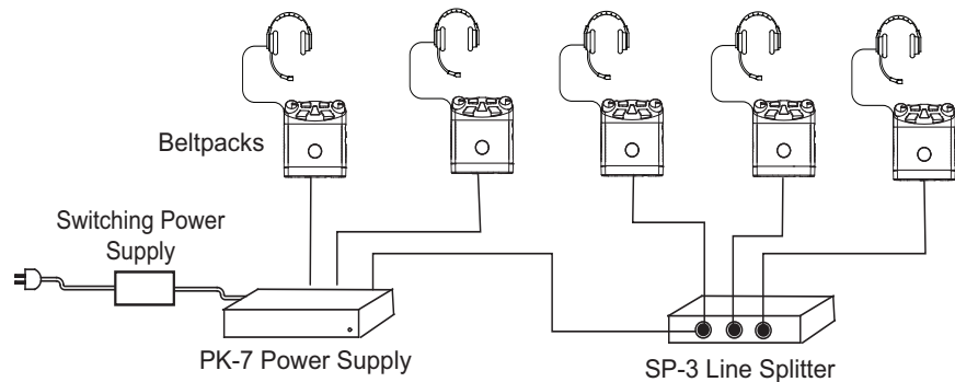
Figure 1-3: Typical System
