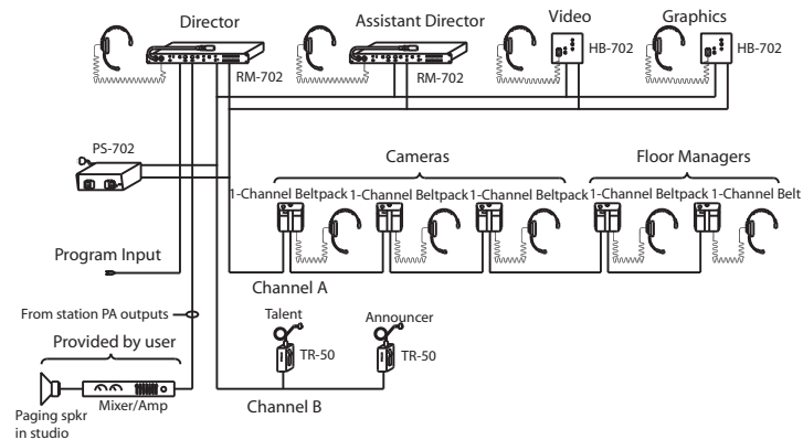
Figure 2-11: Typical Cable or School Television Studio Installation
