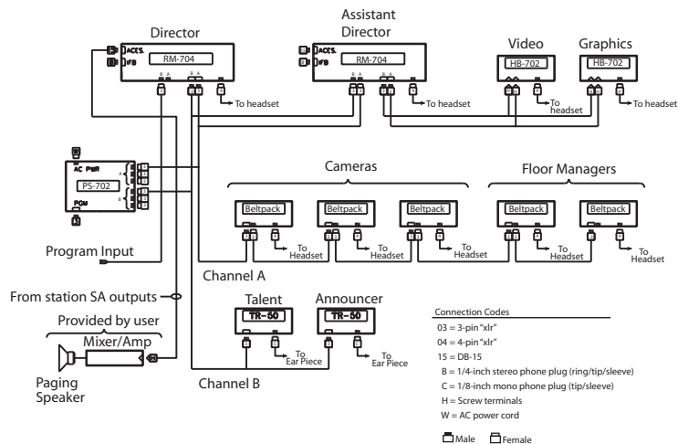
Figure 2-12: Connecting a Small Cable/School Television Studio
