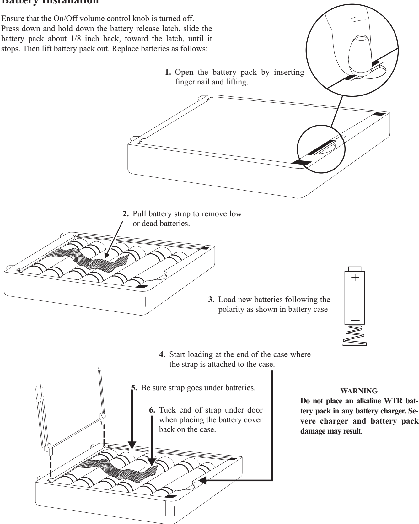
Figure 18 Battery Installation
