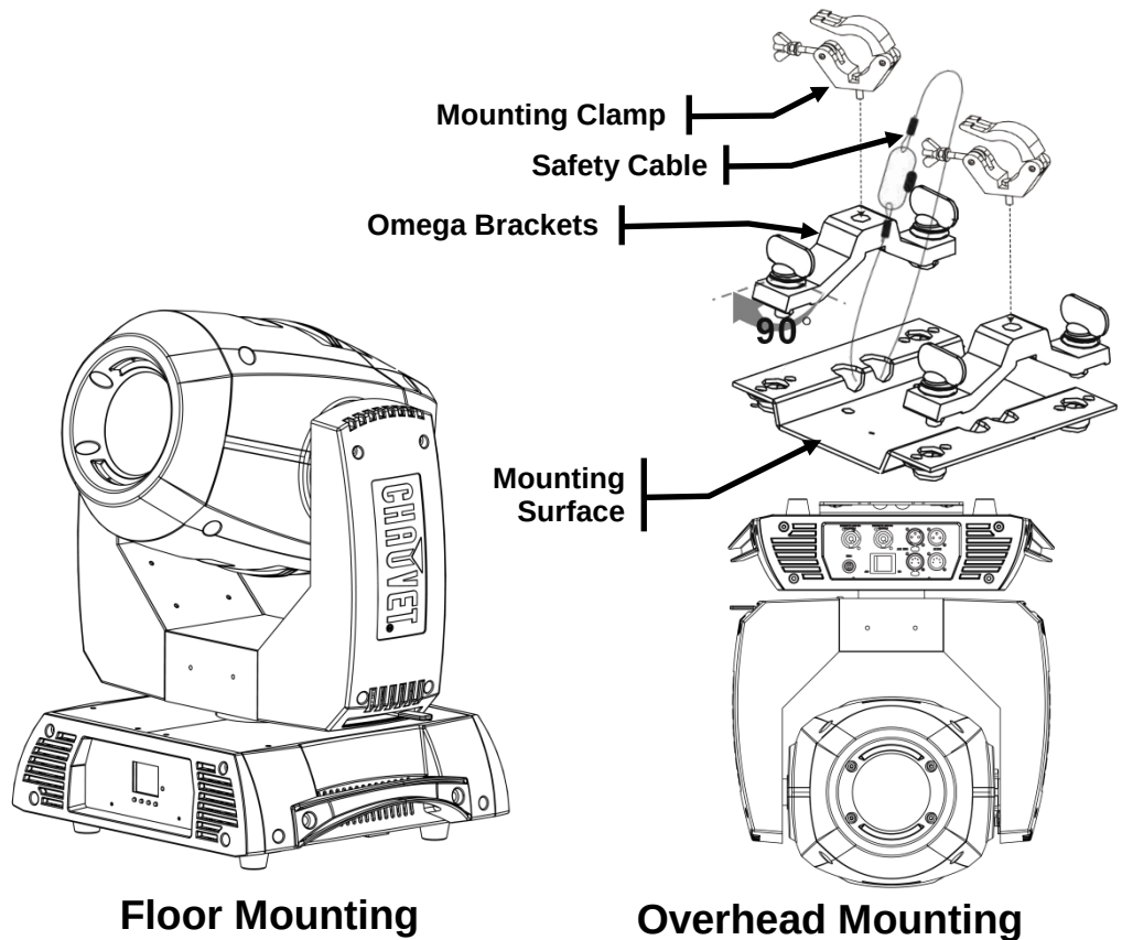
Mounting Diagram
