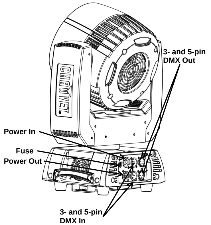
Rear View
