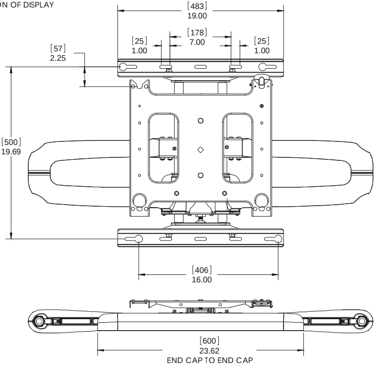
Mounting Pattern
