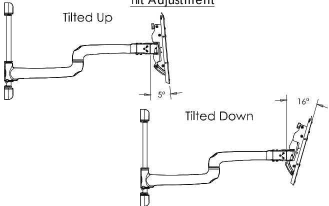
Tilt Adjustment *
