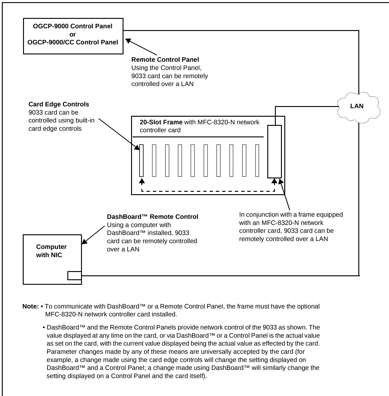
Figure 1-7 9033 User Control Interface
