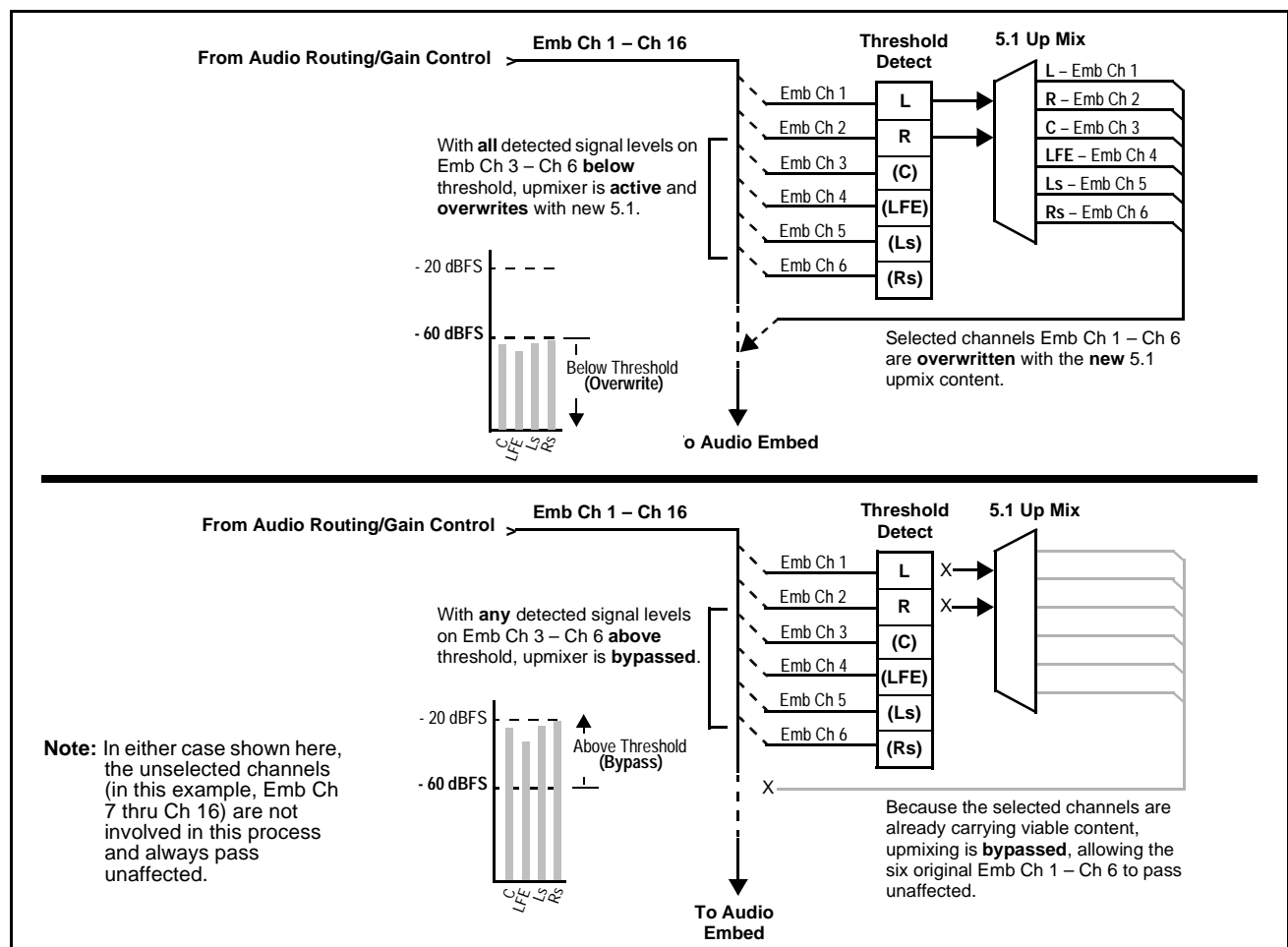
Figure 1-3 Up Mix Auto Enable/Bypass with Example Sources
