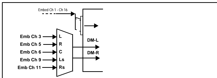
Figure 1-2 Audio Down Mix Functional Block Diagram with Example Sources
