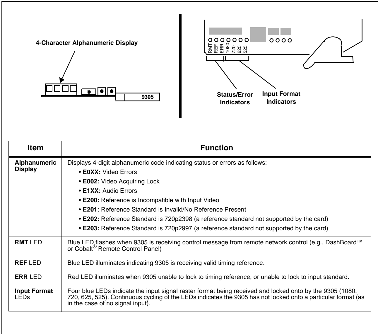
Figure 3-6 9305 Card Edge Status Indicators
