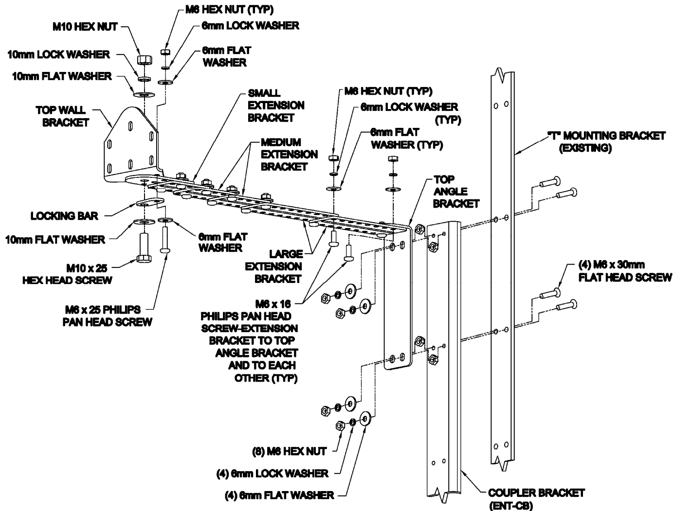
Figure 11: Pan-Tilt Bracket - Top Assembly
