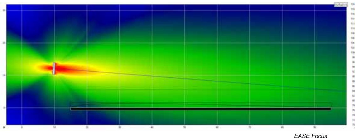
Figure 26: One Full-Range Column (1 kHz)
