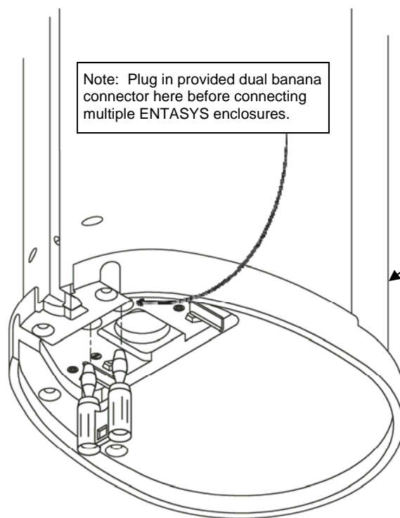
Figure 23: ENTASYS Dual Banana Plug Jumper
