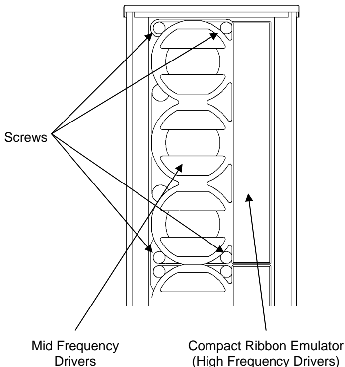
Figure 24: ENTASYS MF/HF Module Screw Locations
