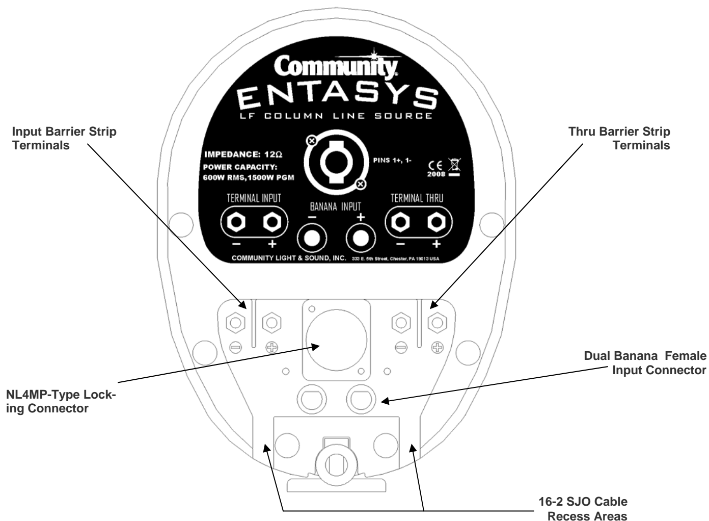
Figure 20: ENTASYS Low Frequency Column Input Panel
