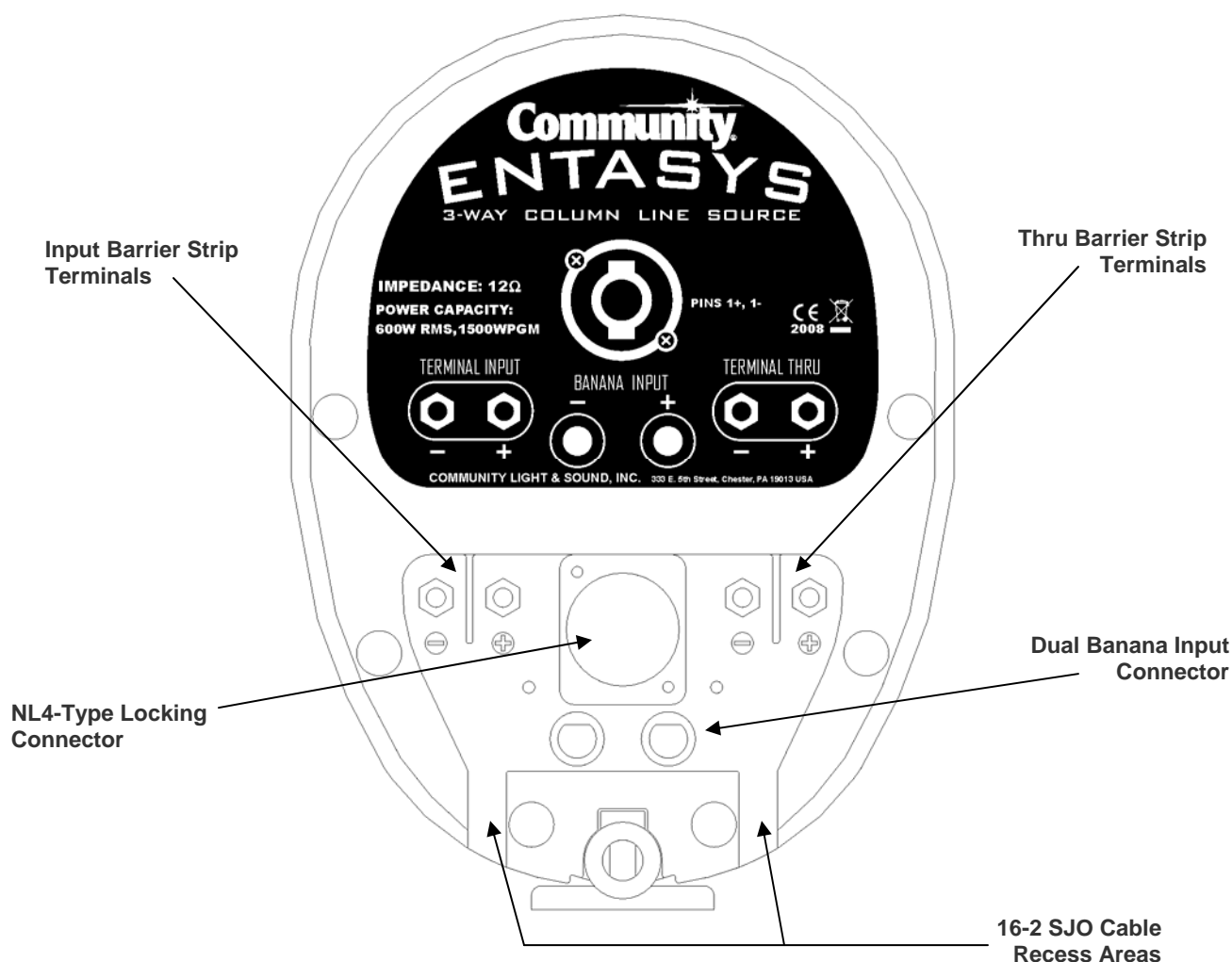
Figure 19: ENTASYS Full-Range Column Input Panel
