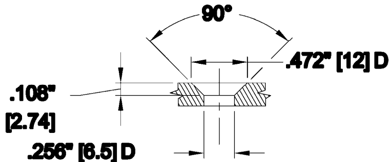
Figure 5: Countersink Detail
