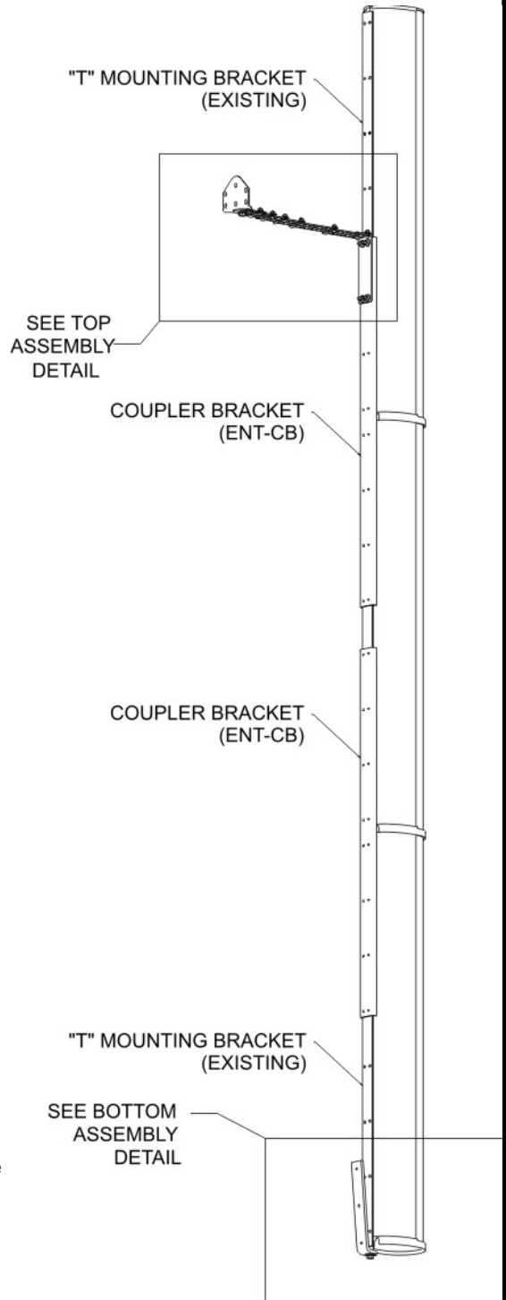
Figure 10: Pan-Tilt Bracket on Multiple Columns
