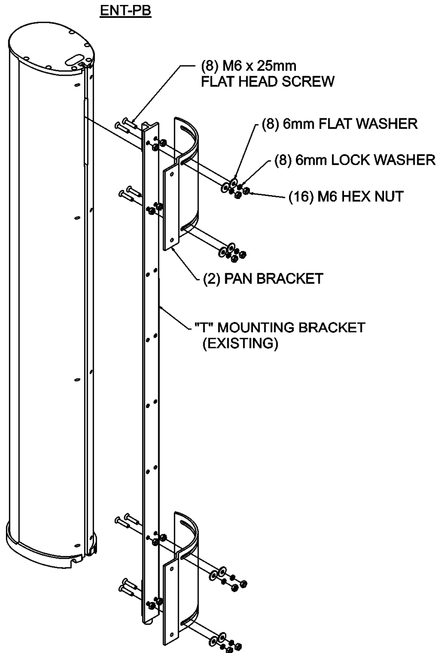
Figure 9: Pan Bracket
