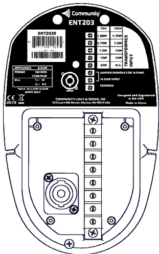
BOTTOM showing input connectors (typical)
