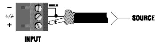
Figure 3.4 Unbalanced Input Connector Wiring
