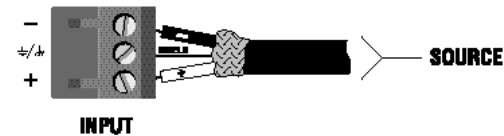
Figure 3.3 Balanced Input Connector Wiring
