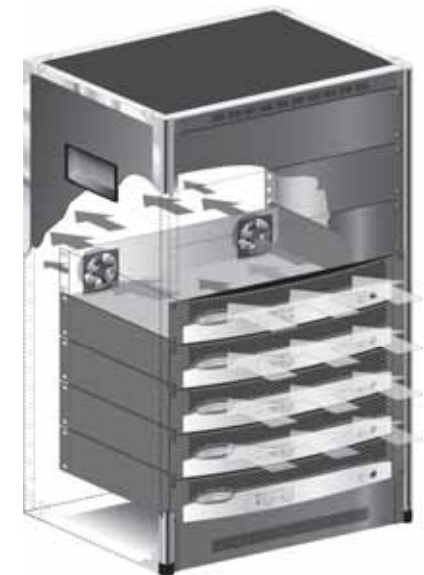
Figure 3.2 Airflow
