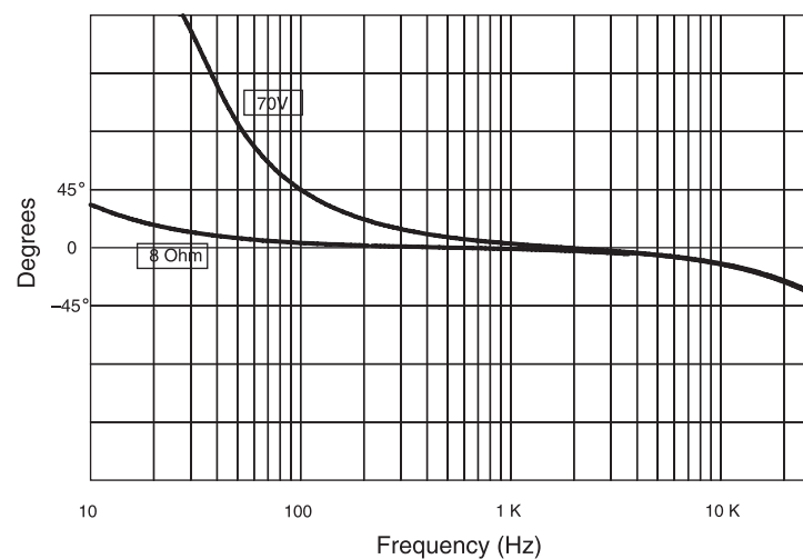
Figure 7.4 CTs 8200 Typical Phase Response (1 W)
