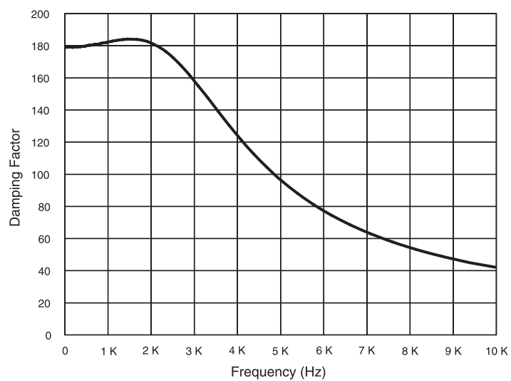
Figure 7.5 CTs 8200 Typical Damping Factor vs. Frequency
