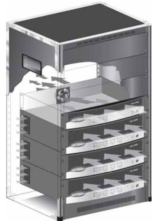
Figure 3.2 Airflow
