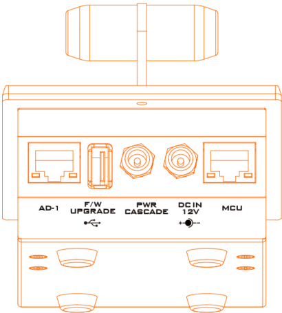
RJ-45 Port (AD1) Connection to AD1
