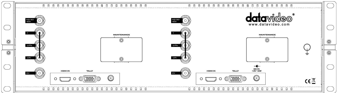
HD/SD - SDI input BNC connector for SDI Input.
