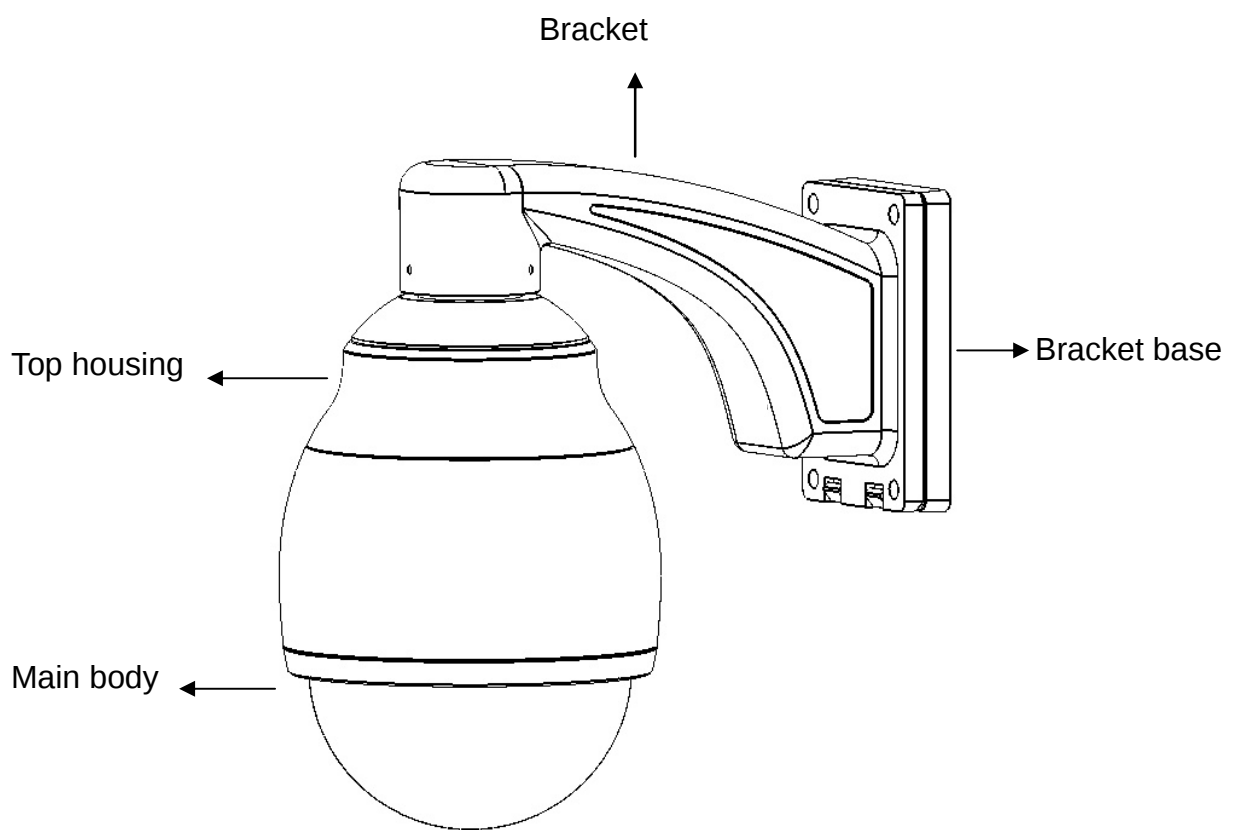
ETPZ3100 overview
