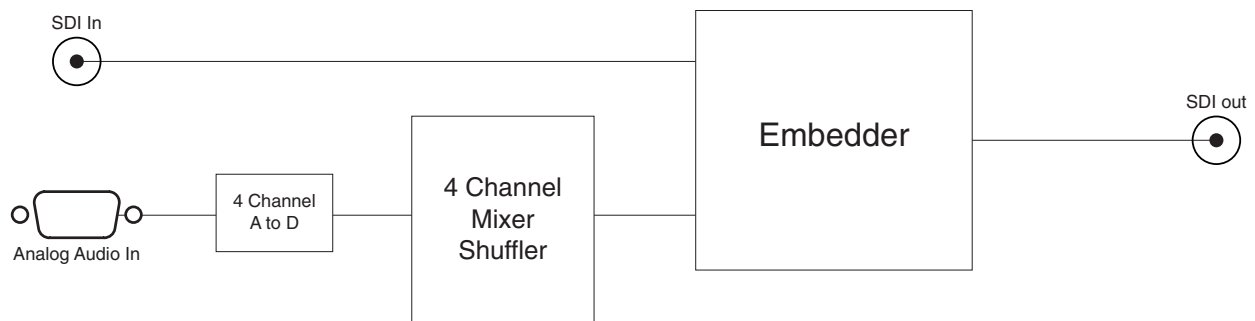
BrightEye 23 Functional Block Diagram
