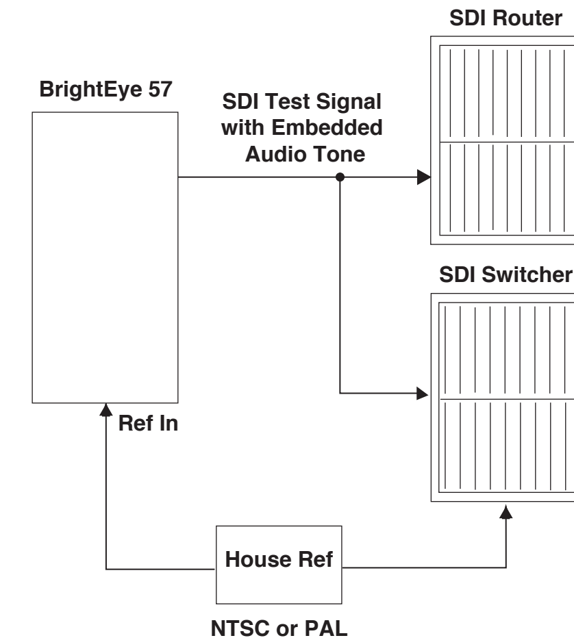
BrightEye 57 Genlocked Test Signal Application
