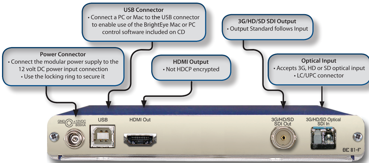
BrightEye 81-F Rear View
