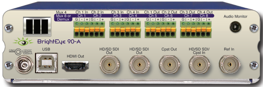
BrightEye 90-A Rear Connectors
