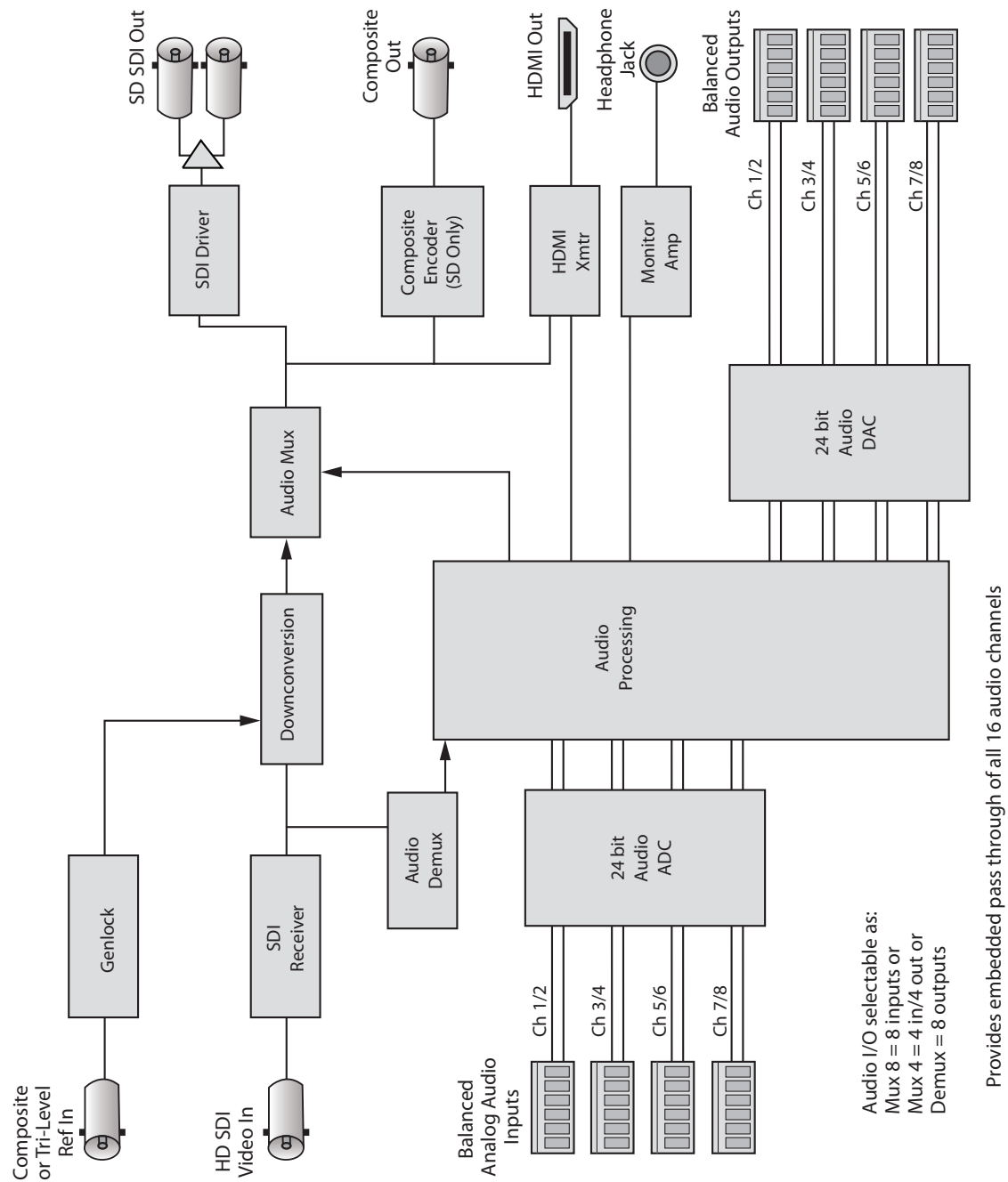
BrightEye 92-A Functional Block Diagram, landscape view
