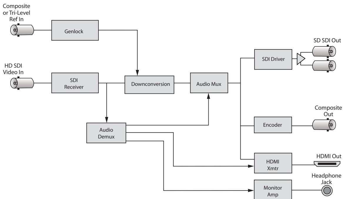
BrightEye 92-M Functional Block Diagram
