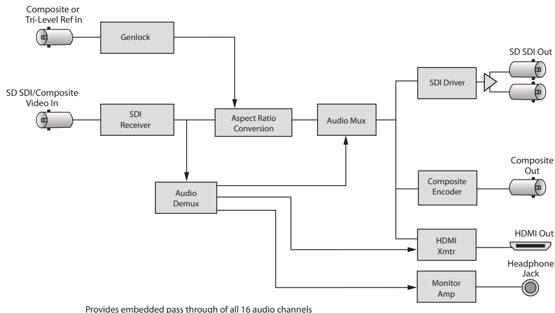
BrightEye 94 Functional Block Diagram, portrait view
