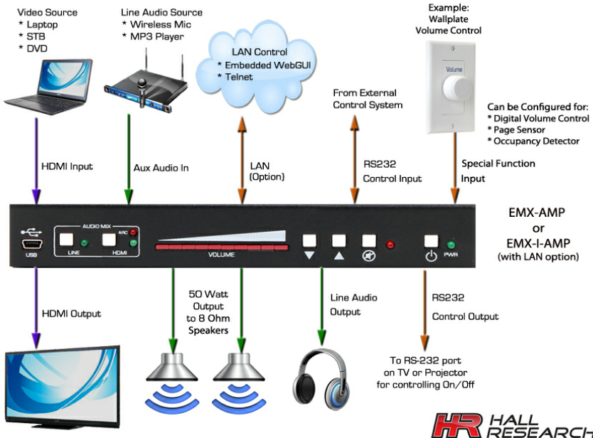
Figure 1 – Connection Diagram
