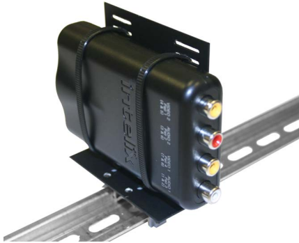
One Intelix AVO-V1A2 balun mounted to an Intelix AVO-CLIP on a 35 mm DIN rail.
