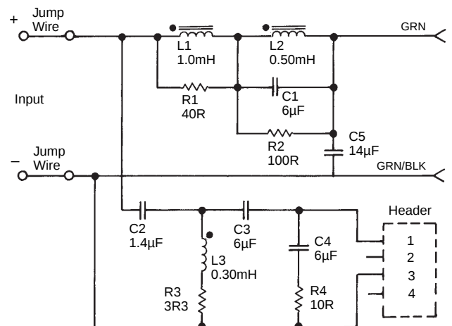
SCHEMATIC (129-20049-00)
