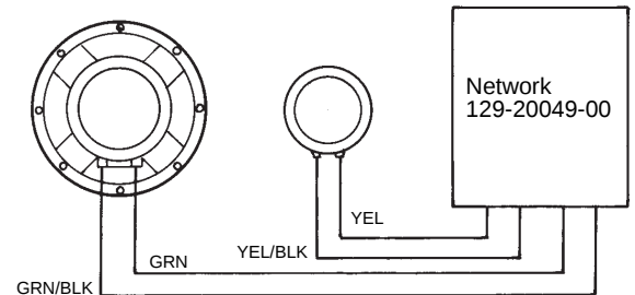
SCHEMATIC (129-20049-00)
