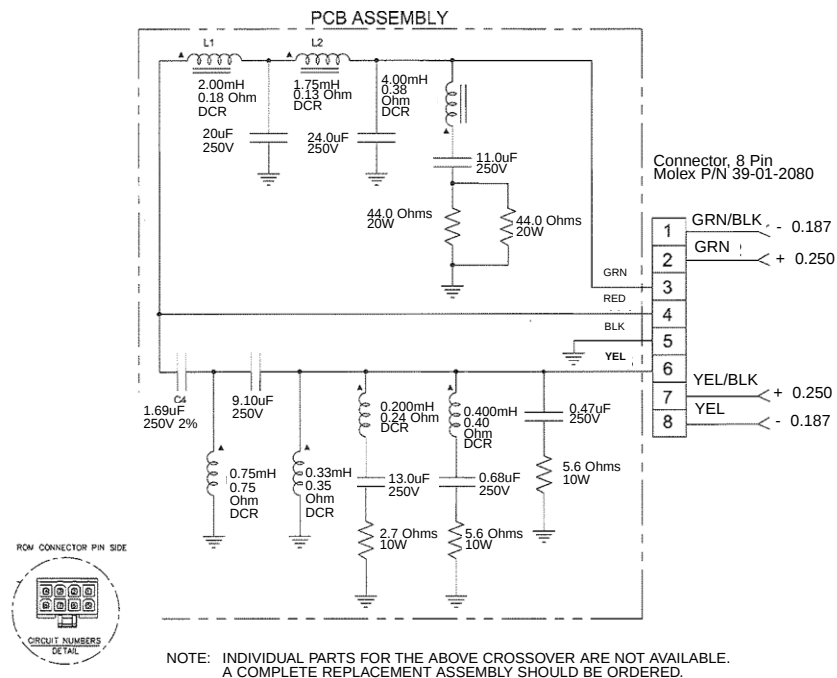
Network Assembly Schematic - 443748-001
