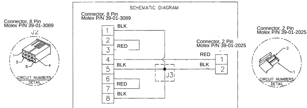
Wire Harness Schematic Diagram - 446150-001
