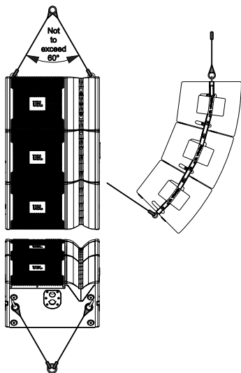
EYEBOLT SUSPENSION
