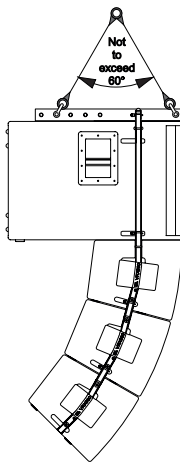
ARRAY FRAME SUSPENSION
