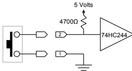
GPI Input Example with Pushbutton Switch
