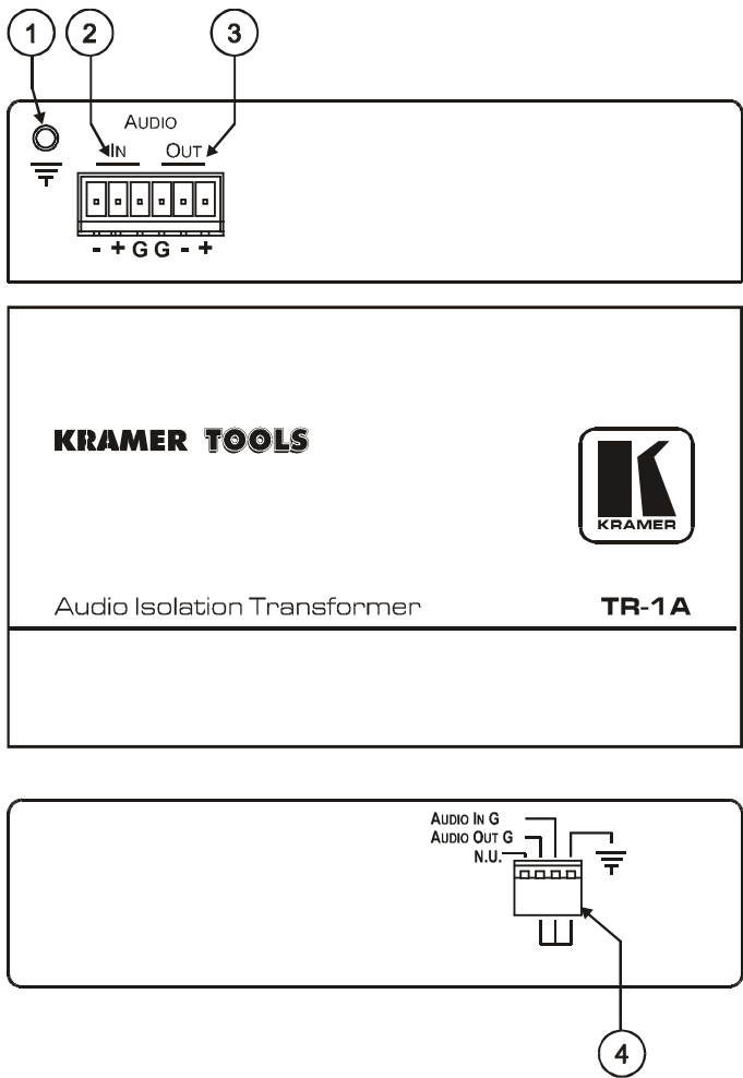
Figure 2: TR-1A Audio Isolation Transformer
