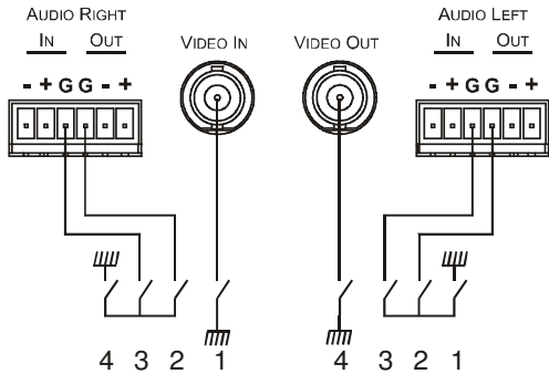
Figure 7: IN and OUT Grounding Options
