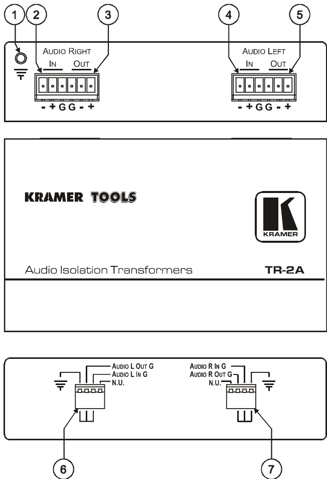
Figure 3: TR-2A Audio Isolation Transformers
