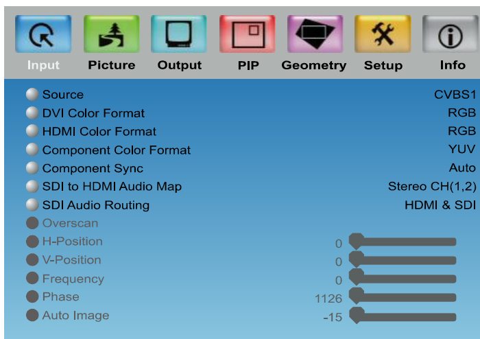
Figure 5: Input Screen
