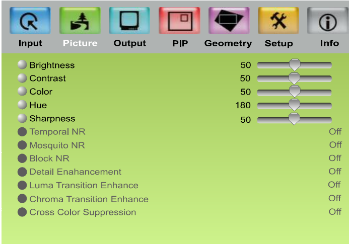
Figure 6: Picture Screen
