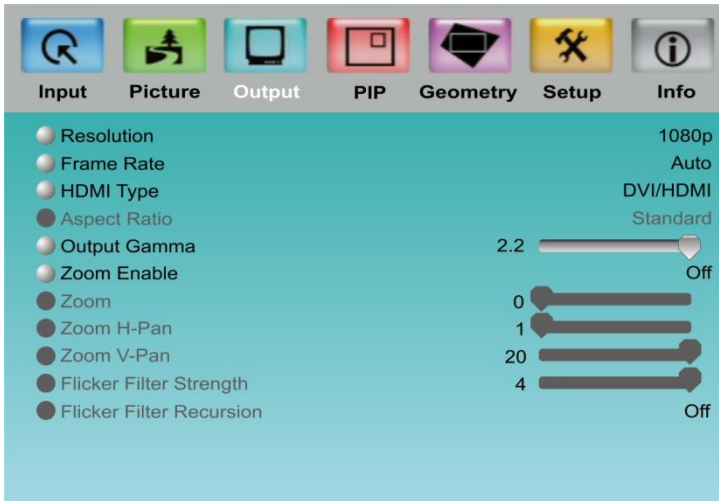
Figure 7: Output Screen
