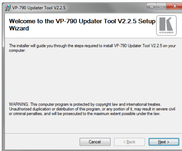
Figure 20: Welcome Window
