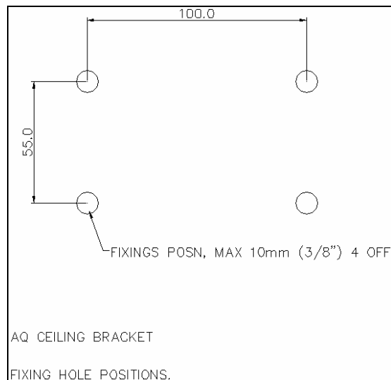
AQCS AQCL Ceiling Brackets – AQCS (short) for AQ8, AQ10, AQCL (long) for AQ8, AQ10, AQ12
