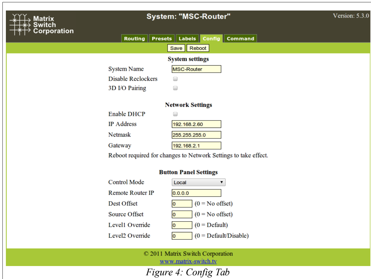
Figure 4 depicts the Config Tab as seen on a Router system beginning with Carina Series Firmware 5.3.0. Configuration fields vary depending on router features, firmware version and if the device is a Remote Panel.
