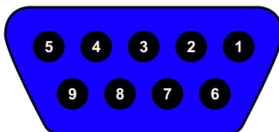
DE-9 Pinout
