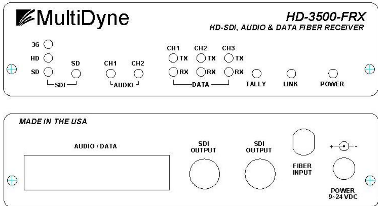
Figure 3. Front and Back of HD-3500-FRX
