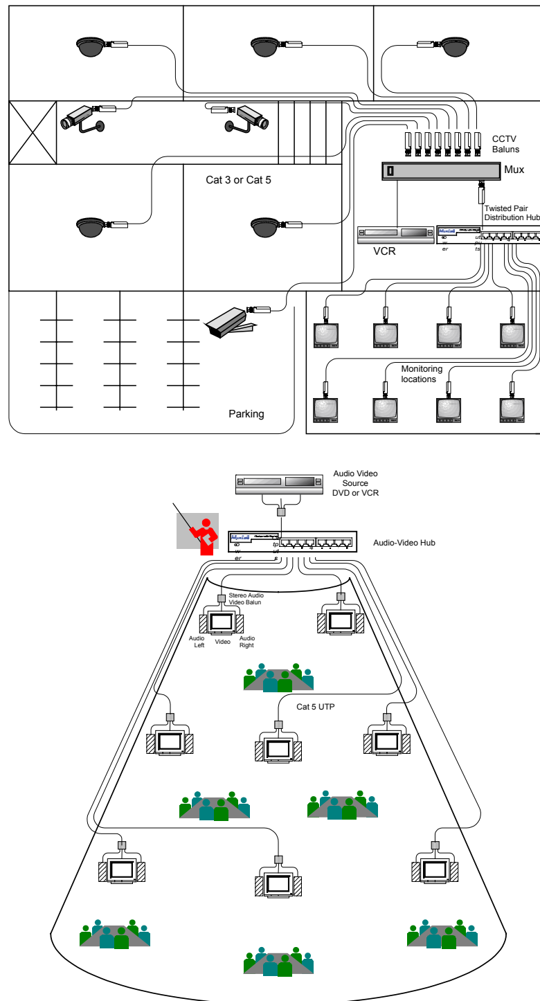
Figure 6 : Typical Installations
