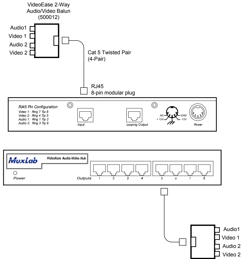
Figure 5 : Connection Diagram
