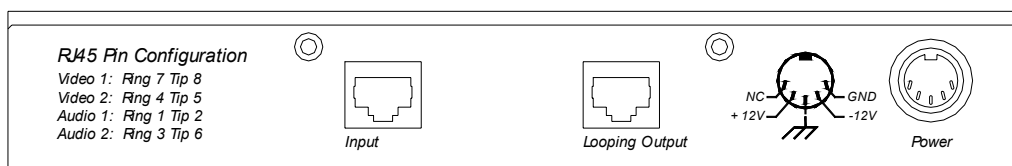
Figure 3 : Audio-Video Hub Back Panel
