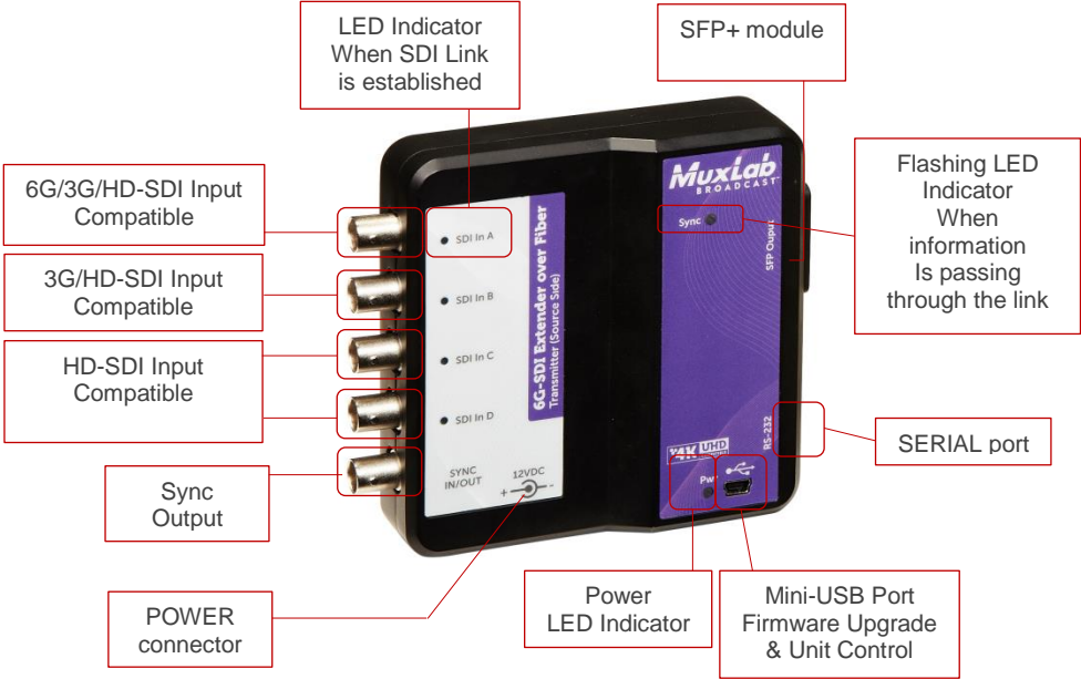
Figure 2 Front View of Transmitter
