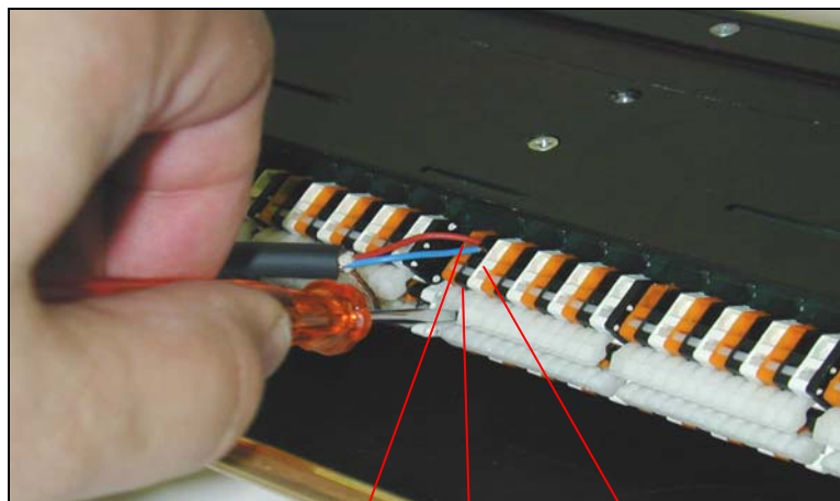
Tip Ring Sleeve
