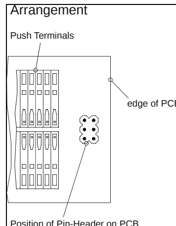
Pin Header
