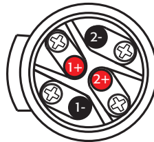
Male NL4 Wiring
