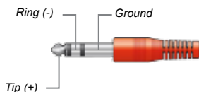
Balanced TRS \frac{1}{4} " Phone
