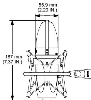
FIGURE 6. DIMENSIONS
