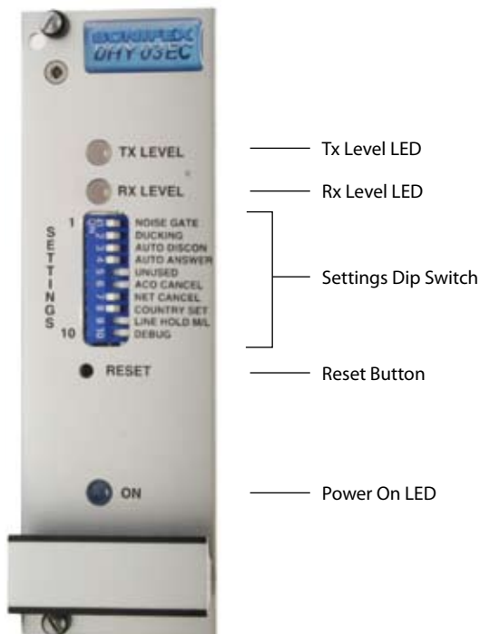
Figure 2-6 : DHY-03EC Controls.
