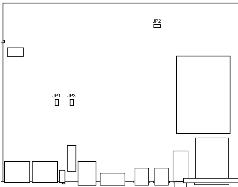
Figure 2-5 : PCB Layout.
