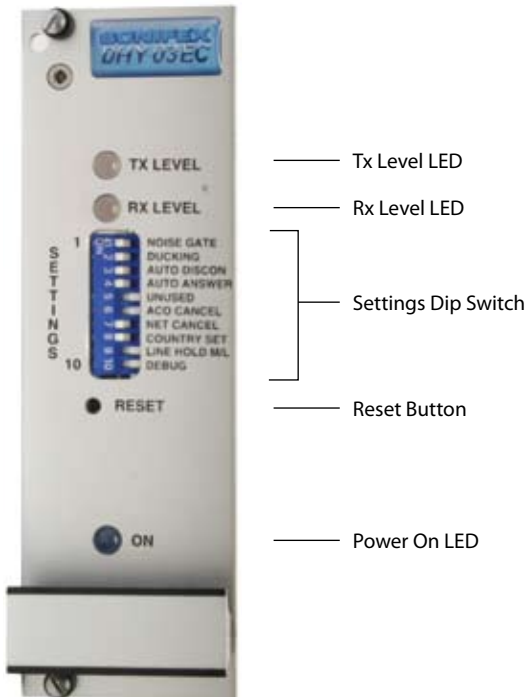
Figure 2-6 : DHY-03EC Controls.
