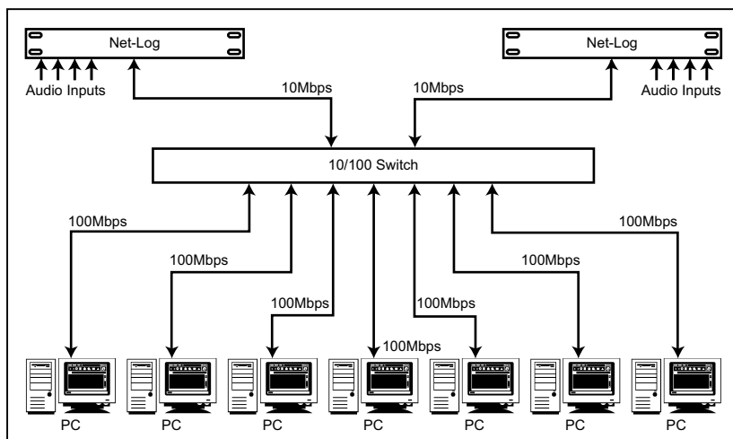
Fig 3-1: Network Topology.
