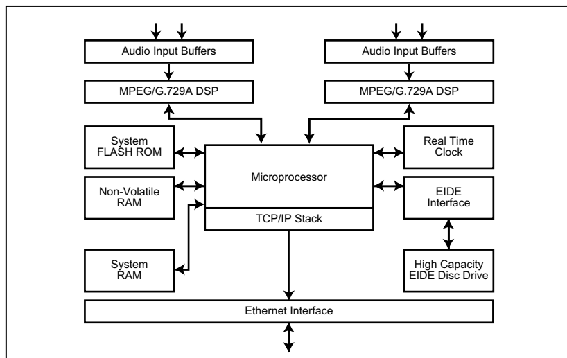
Fig 1-1: Net-Log System Block Diagram.
