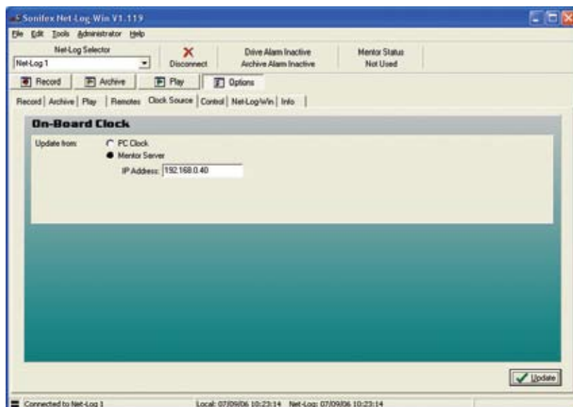
Fig 9-5: Clock Source Options.
